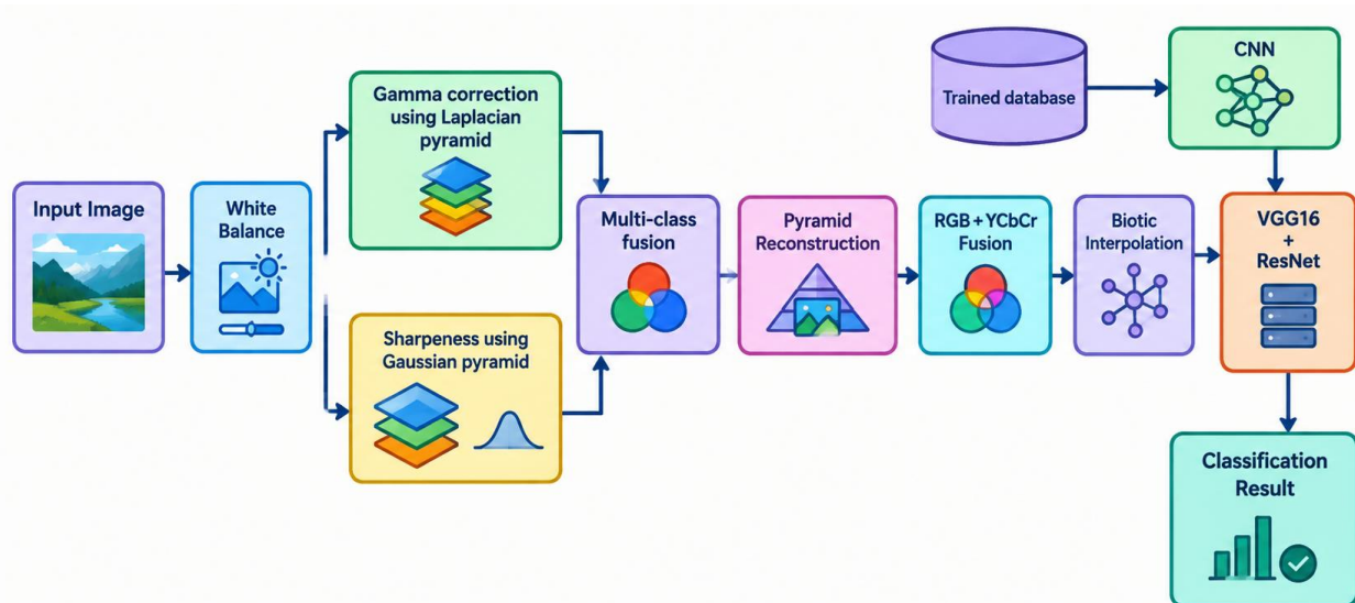
Figure 2: A block diagram illustrating the proposed DLCNN's step-by-step execution using MEF
