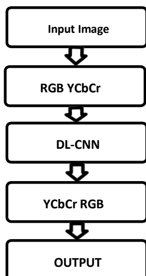
Figure. 3 Flowchart of DLCNN
