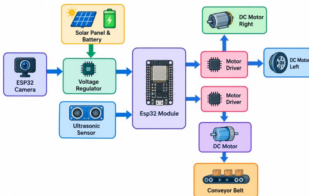
Figure.2 General Block Diagram
