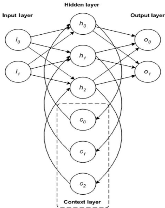
Figure.1 Recurrent Neural Networks (RNNs)
