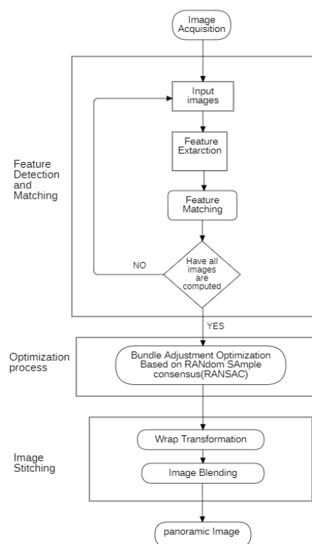
Fig.1 Architecture
