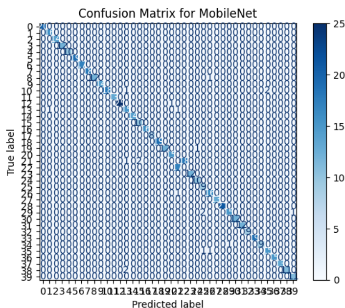
Figure.3 MobileNet Confusion Matrix
