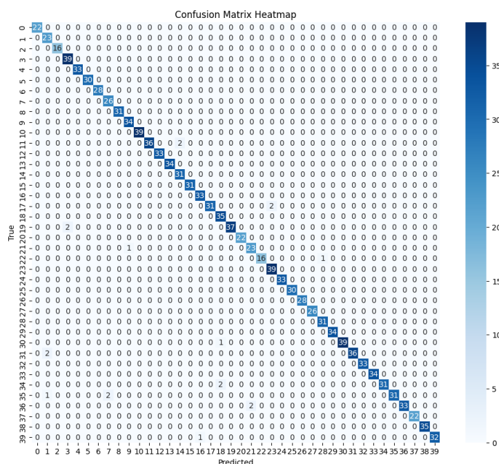
Figure 4 MobileNet + RNN confusion Matrix
