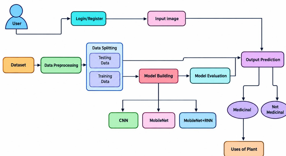
Figure.1 Proposed System Flow
