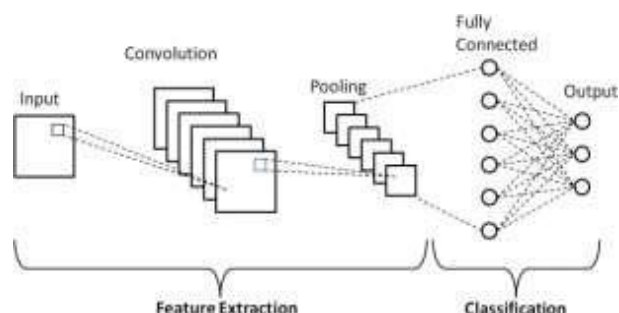
Figure. 2 CNN architecture
