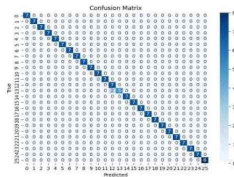
Figure. 5 Confusion Matrix for CNN
