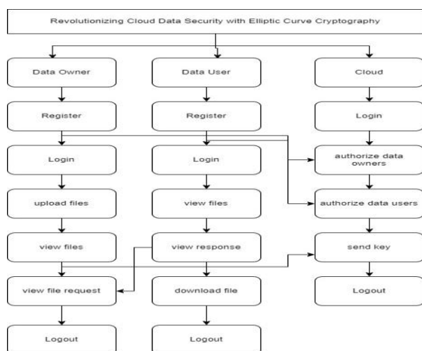
Figure.2 Flow chart of Advancing Cloud Data Protection with Cryptographic Algorithms
