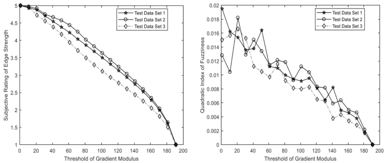
Figure.6: Neuron Analysis
