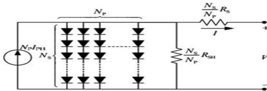
Figure. 3 Equivalent circuit of solar array.
