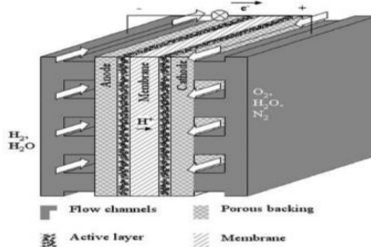
Fig. 4 Model representation of a proton exchange membrane fuel cell.
