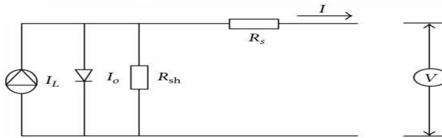
Figure. 2 PV cell equivalent circuit
