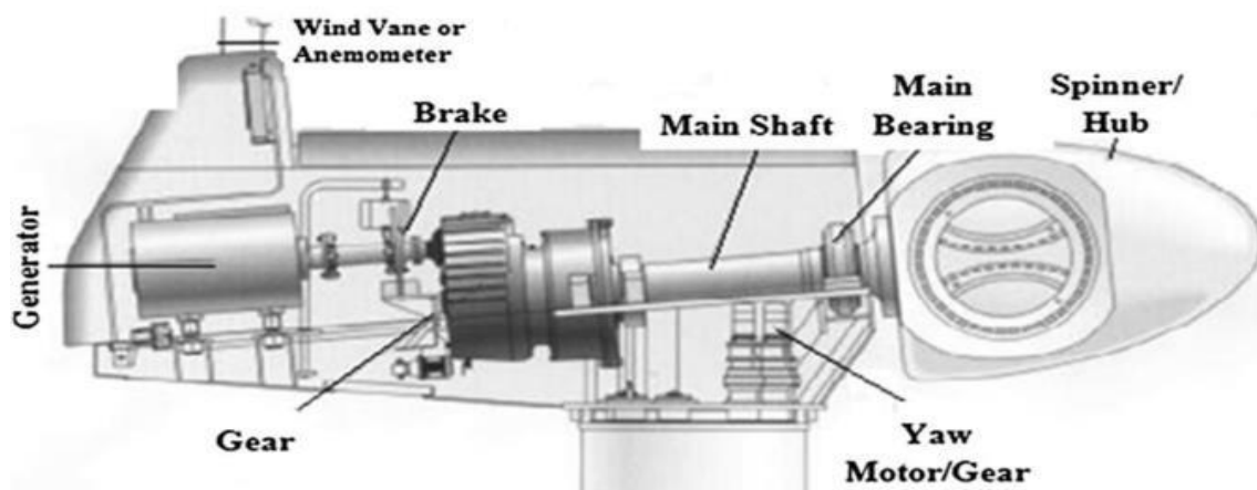
Figure. 3 Cross section showing the arrangement of internal parts of a wind turbine
