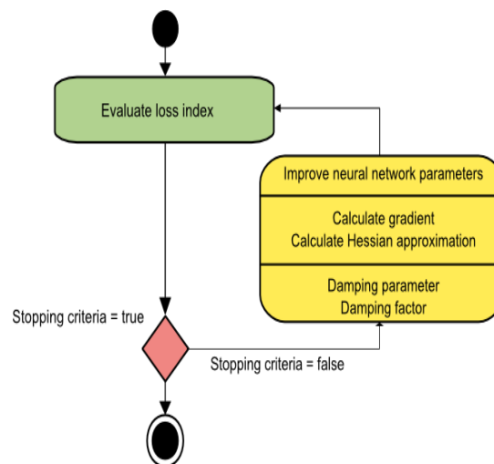
Figure.5 Workflow Mechanism
