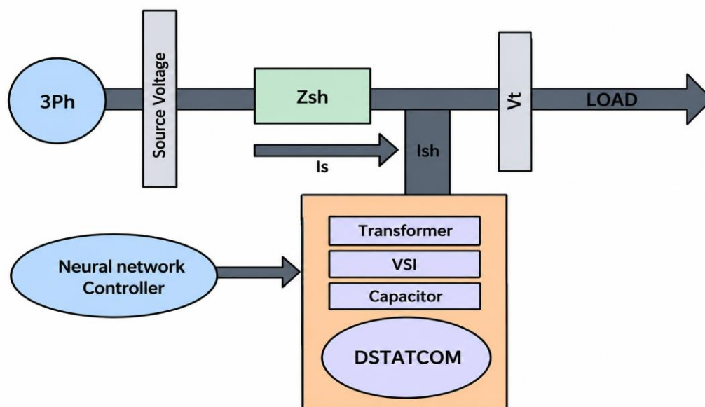
Fig. 1 Diagram of the power model with DSTATCOM.
