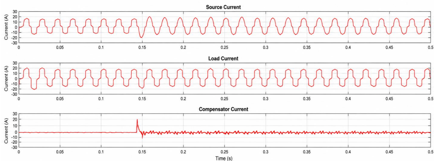
Fig 3. (a)Source current (b) Load current (c)Injected current
