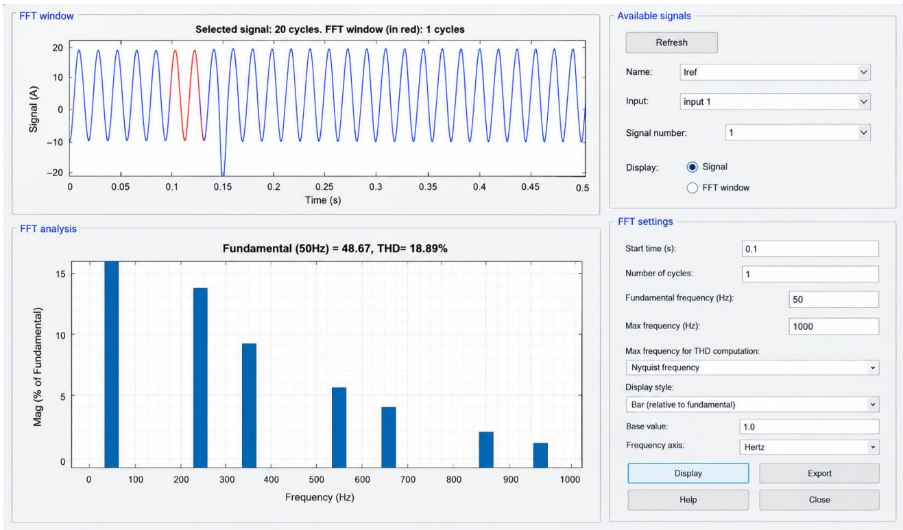
Fig.4 Source current THD% (18.88%) before compensation
