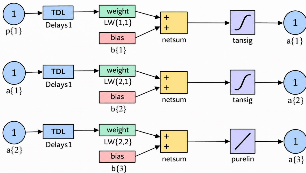
Fig. 2 Neuron in matrix form at each layer
