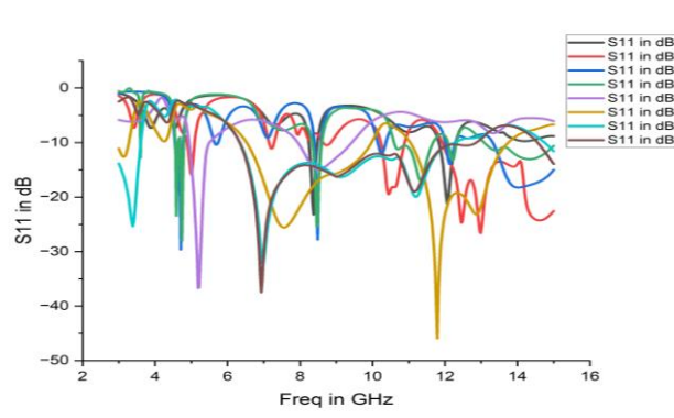
Figure. 11 reflection coefficient plots of all phase antennas
