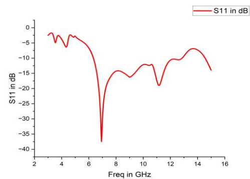
Figure.2 S11 plot of Elliptical Slot Antenna with DGS
