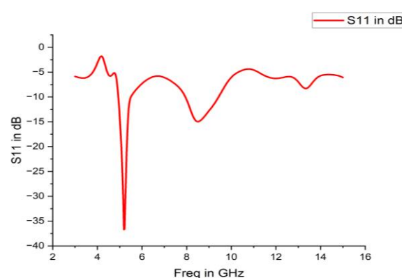
Figure.8 S11 plot of Defected Ground Structure
