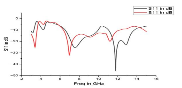
Figure.10 S11 plots of Ground Slot Loaded DGS Antenna
