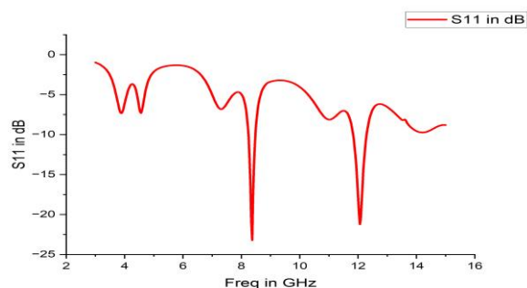
Figure.4 S11 plot of elliptical Antenna
