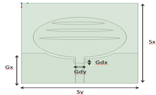
Figure.1 Elliptical Slot Antenna with DGS
