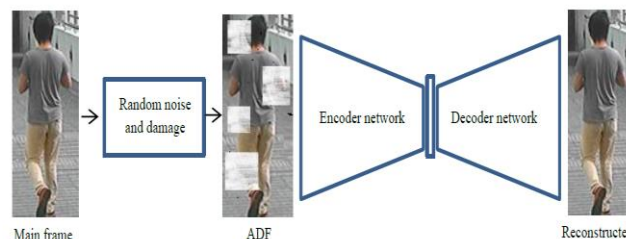
Figure. 2 The idea of Auto Encoder training and ADF for structure reconstruction
