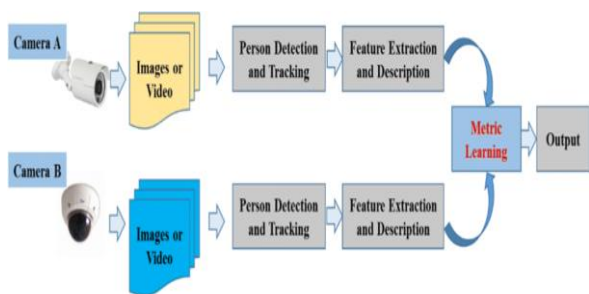
Figure. 4 Block diagram of deep learning CNN
