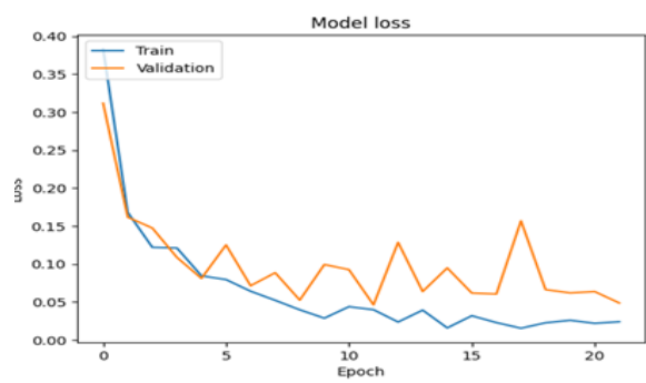
Figure.1 Plot of loss vs validation loss while training
