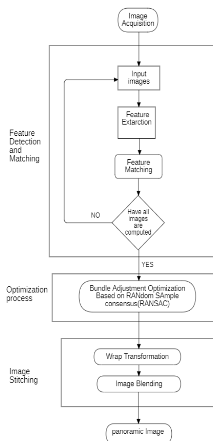
Fig.1 Architecture
